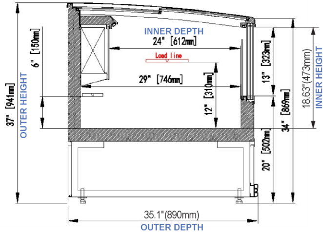
Cross Section:
